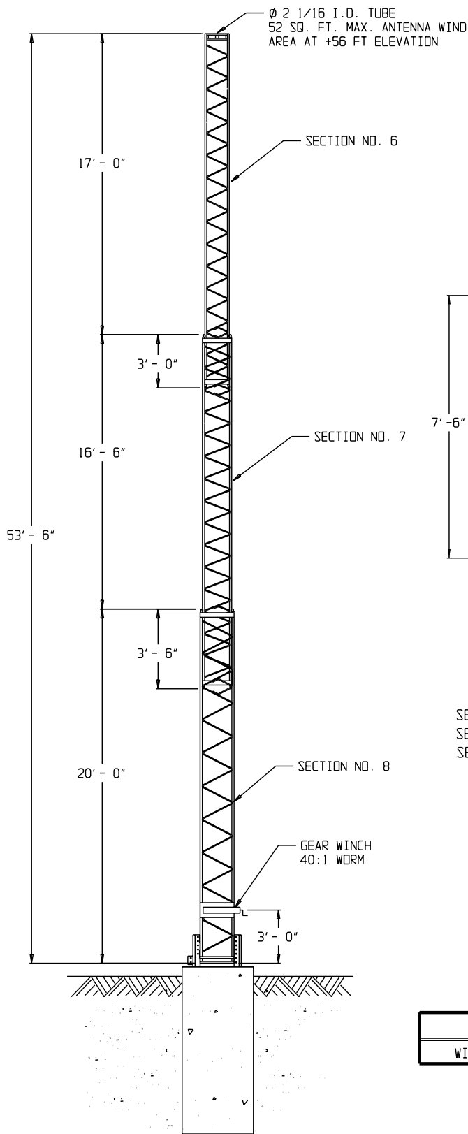
TOWER CROSS SECTION
